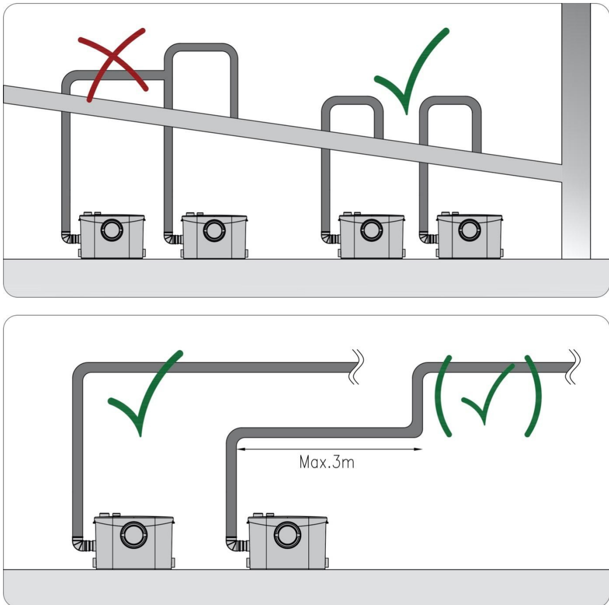
Fig 13 &14: Discharge Pipe connection
